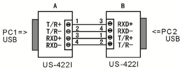
3. Full duplex connection between US-422I interface converters
