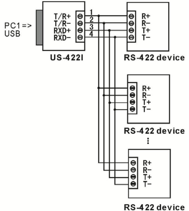
2. RS-422 point-to-multipoint / 4-line full duplex
