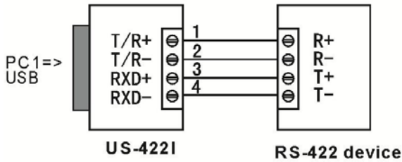
1. RS-422 point-to-point / 4-line full duplex
